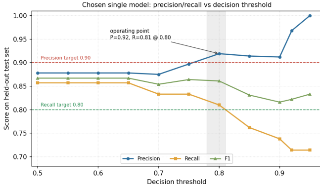
Fig. 2. Precision, recall, and F1 of the chosen single model on the held-out test set as a function of the decision threshold. A threshold near 0.80 satisfies both operating targets, reaching precision 0.92 at recall 0.81, the operating point adopted for full-corpus inference.
