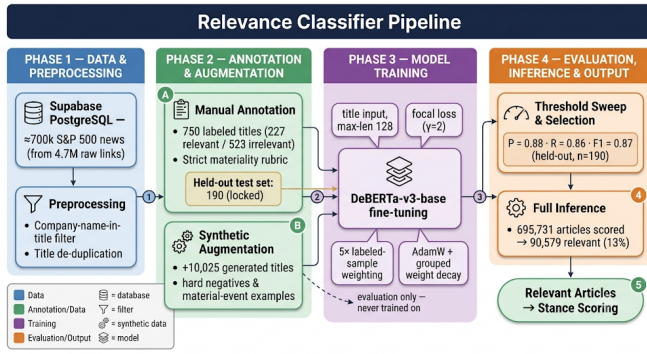
Fig. 1. Relevance classifier pipeline: raw S&P 500 news titles, preprocessing, manual annotation and synthetic augmentation, DeBERTa-v3 fine-tuning, threshold selection on a held-out test set, and full-corpus inference.
